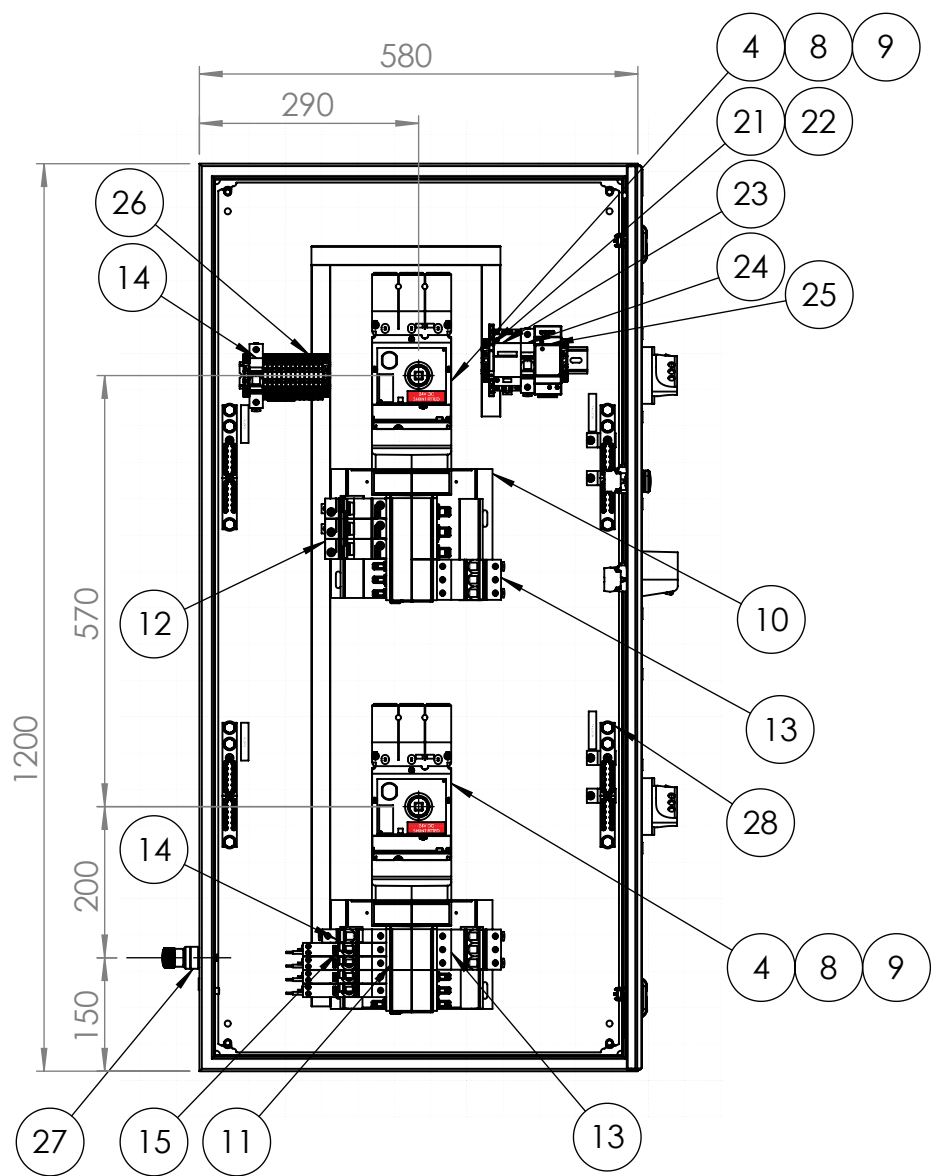
FRONT VIEW
